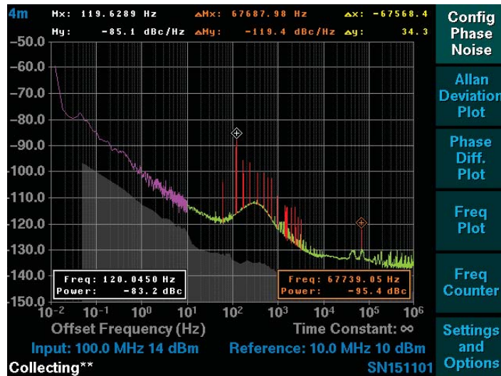
5125A Sample Display Capture – Phase Noise
